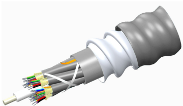
TeraSPEED® Plenum Distribution Cable, interlocking aluminum armored with plenum jacket, 36 fiber multi-unit with 12 fiber subunits
