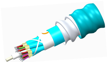
LazrSPEED® Plenum Distribution Cable Interlocking Aluminum Armored with Plenum Jacket 6-Fiber Single-Unit
