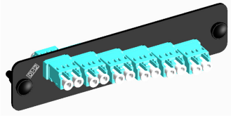
1000-Type Adapter Pack with 6 LC duplex MM adapters, aqua
