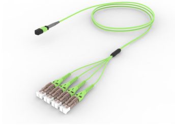
Ultra Low Loss OM5 MPO8 Unpinned to LC/UPC Uniboot 8-Fiber Plenum Array Cord
