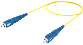
Fiber Optic Patch Cord, Simplex, Singlemode, SC/UPC to SC/UPC, yellow, 3 m
