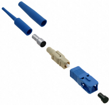
Fiber Optic Connector Kit, singlemode, SC, blue, for 3 mm cable
