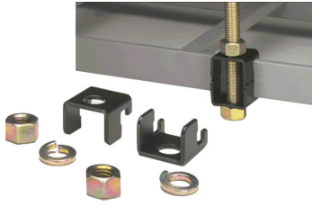
FiberGuide® Ladder Rack Bracket Kit for Radiused Ladder Rake, 5/8in
