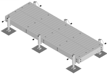
E20® Equipment Platform, 4 ft x 18 ft, base with six adjustable legs
