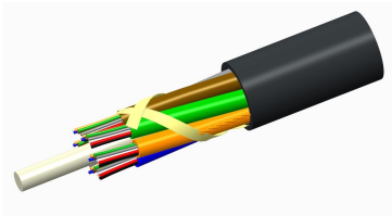
Zero Water Peak,® Blown Micro Single Jacket All-Dielectric Outdoor Stranded Loose Tube 200um Fiber Arid-Core® Construction Cable
