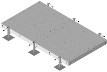
Equipment Platform, 8 ft x 18 ft, base with six adjustable legs
