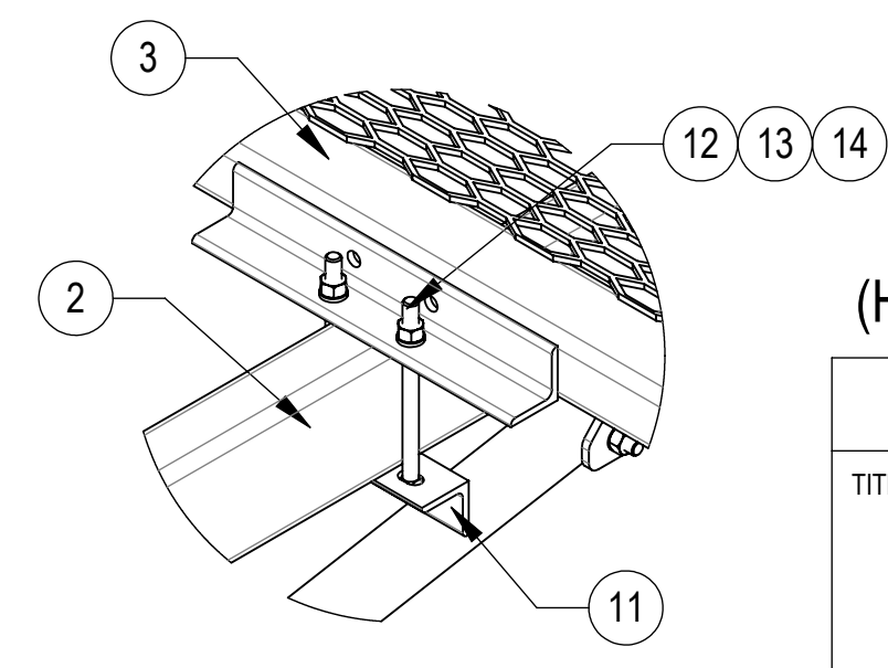
DETAIL E SCALE 1:8
