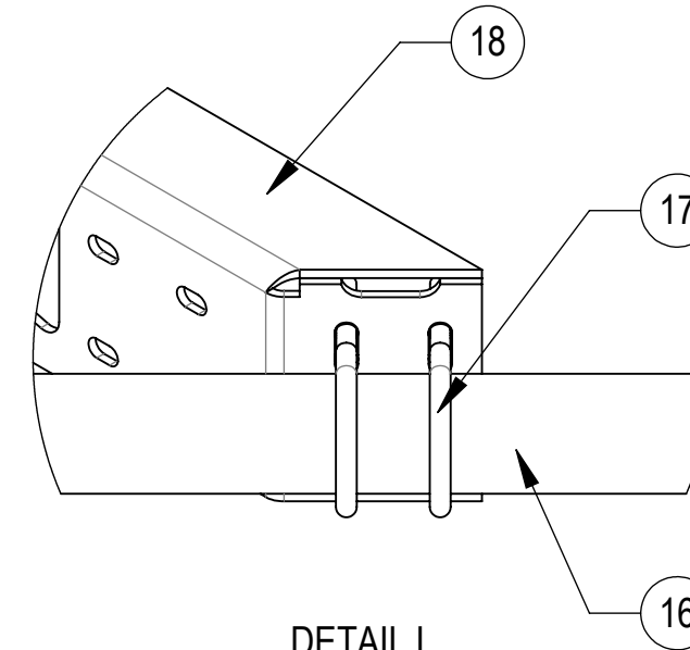
DETAIL L SCALE 1 : 5
